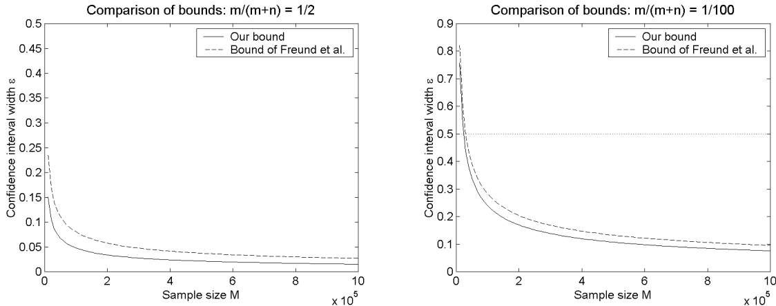
Figure 1: A comparison of our uniform convergence bound with that of [FISS03] for the class of linear ranking functions on \mathbb{R} . The plots are for \delta = 0.01 and show how the confidence interval width \epsilon given by the two bounds varies with the sample size M , for various values of m/(m+n) . In all cases where the bounds are meaningful ( \epsilon < 0.5 ), our bound is tighter.
