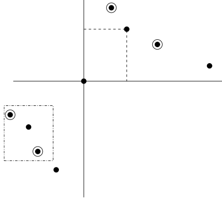
Figure 3: A point p and the neighbors of p in two opposite quadrants in the graph G(P, \mathcal{B}^2) . The doubly-circled points form an independent set in this graph.
