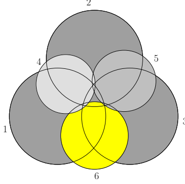
Figure 2: The range space depicted is (V, E_V) , where V is the set of circles \{1, 2, 3, 4, 5, 6\} and every face of the arrangement \mathcal{A}(V) induces a subset in \Phi_V , which is the subset of circles of V covering this face. Clearly, the range \{1, 2, 3\} \in \Phi_V but the ranges \{1, 2\} , \{2, 3\} , \{3, 1\} are not in \Phi_V since there is no face in the arrangement that is covered only by those pairs of circles. Thus, the range space (V, \Phi_V) is not monotone. In particular, the set \{1, 2, 3\} is independent in the graph G(V, E_V) while it is not admissible, and as such the coloring depicted, which is clearly illegal (in the conflict-free sense), is one that Algorithm 1 might output.
