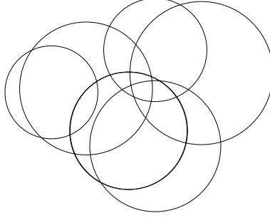
Figure 1: A set \mathcal{S} of discs and an admissible subset \widehat{S} (depicted shaded).
