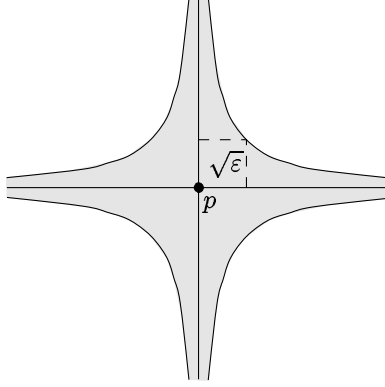
Figure 4: The region S(p, \varepsilon) .
