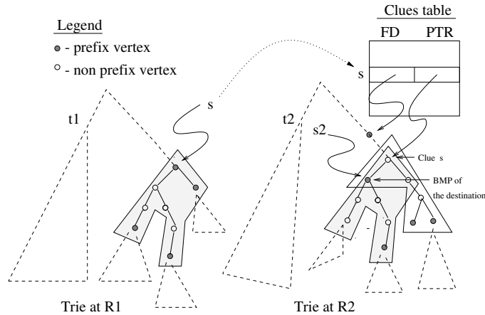
Figure 6: Conditions of the inverse of Claim 1.
