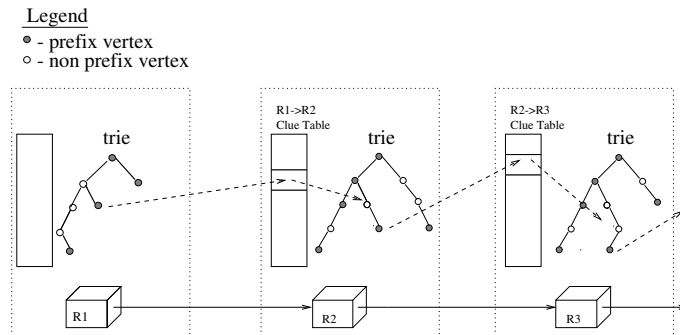
Figure 2: Schematic view of Distributed IP lookup.
